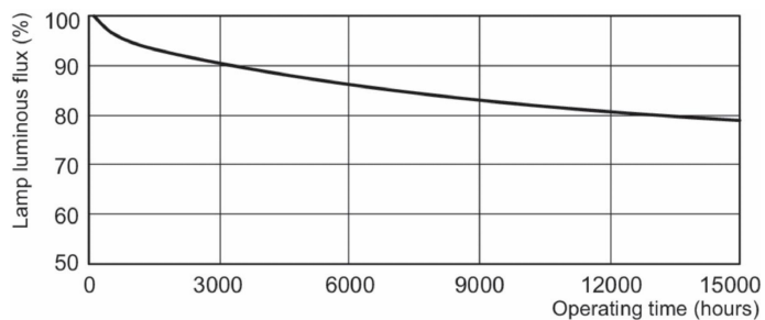
Lumen Maintenance Diagram - PL-C 26W/840/4P 1CT/5X10BOX
